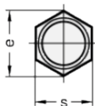
Mounting block GN 412.1
